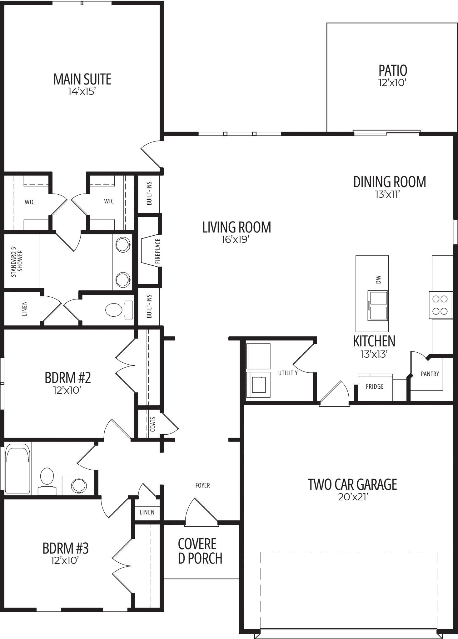
FIRST FLOOR - 1,596 SQ. FT
