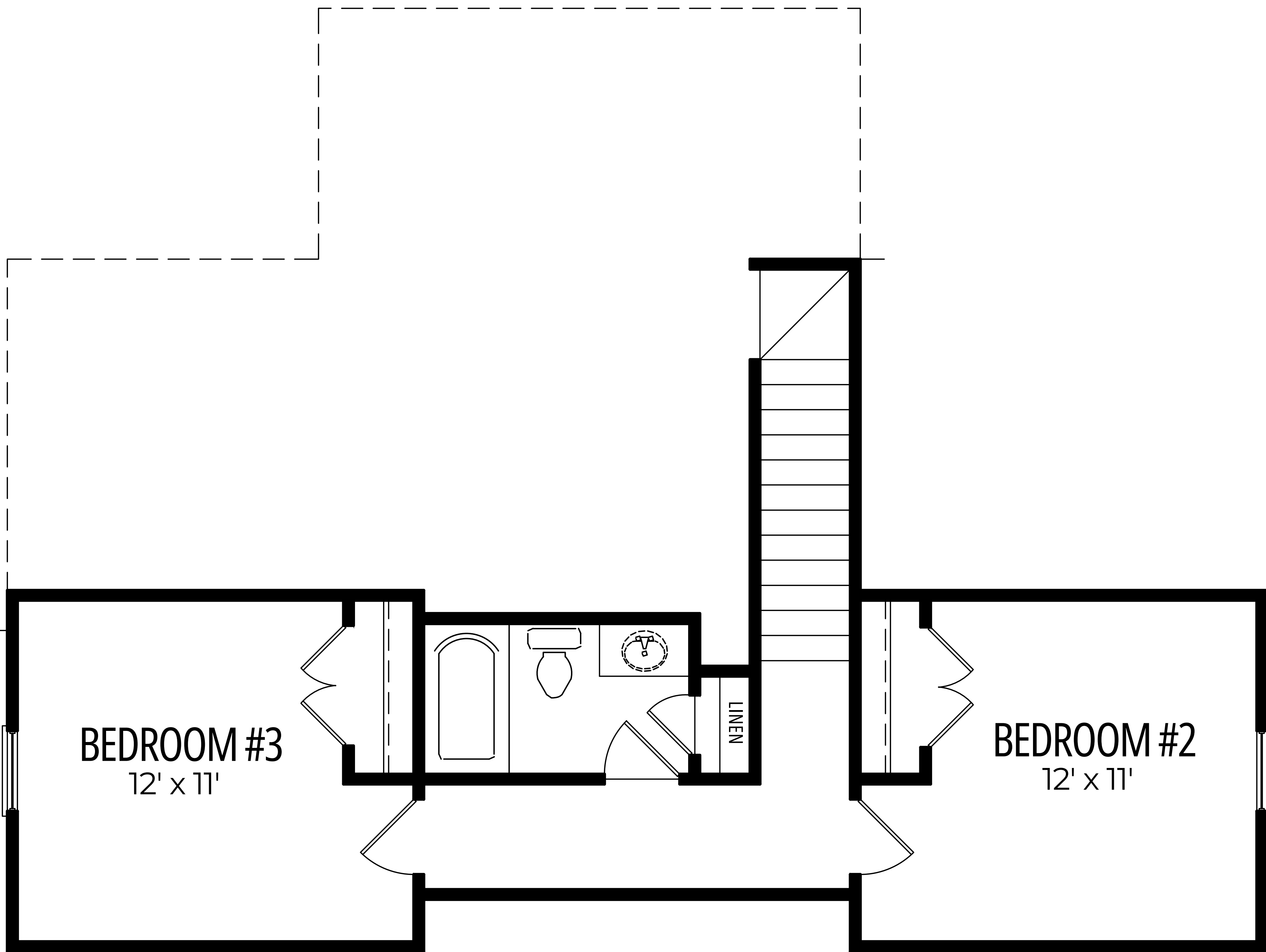
SECOND FLOOR
