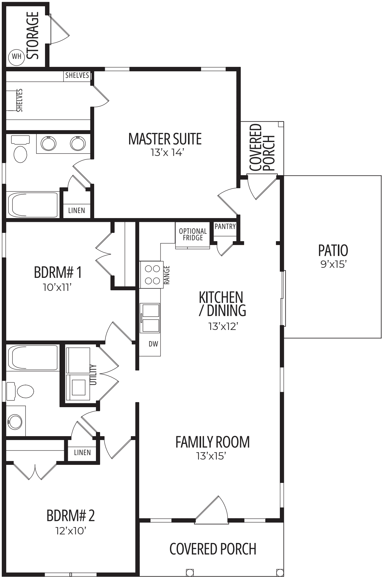
3 Bedroom Option
